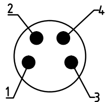
MALE END VIEW
